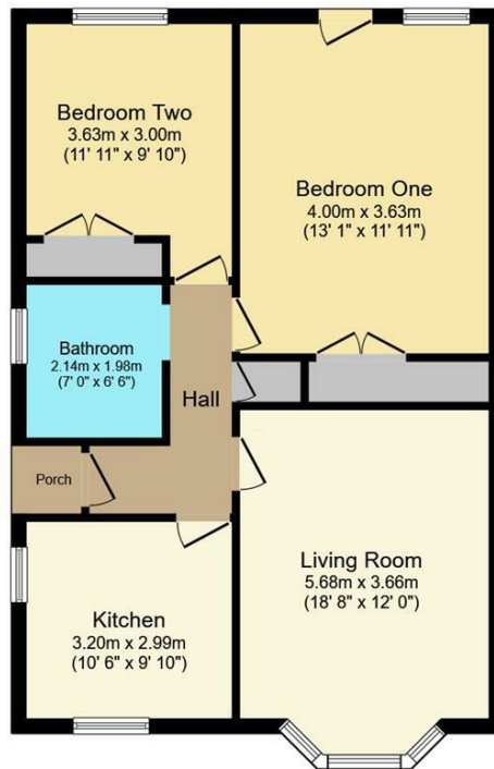
Floor Plan Floor area 68.8 m 2 (741 sq.ft.)
