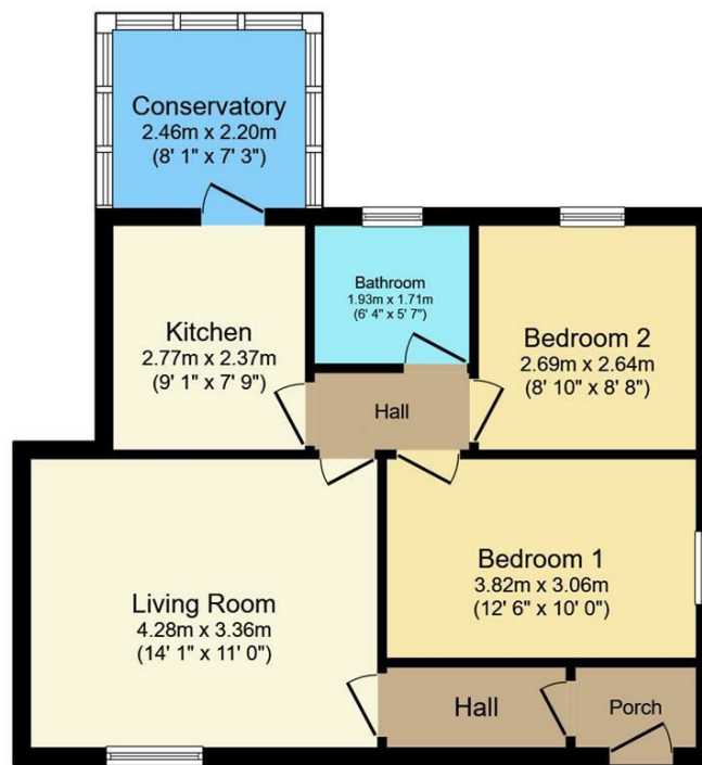
Floor Plan Floor area 55.5 m 2 (598 sq.ft.)
