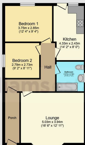
Floor Plan
