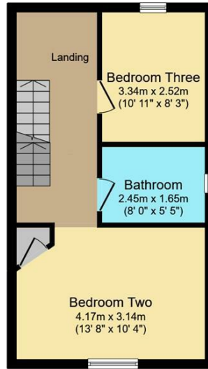
First Floor Floor area 36.6 sq.m. (394 sq.ft.)
