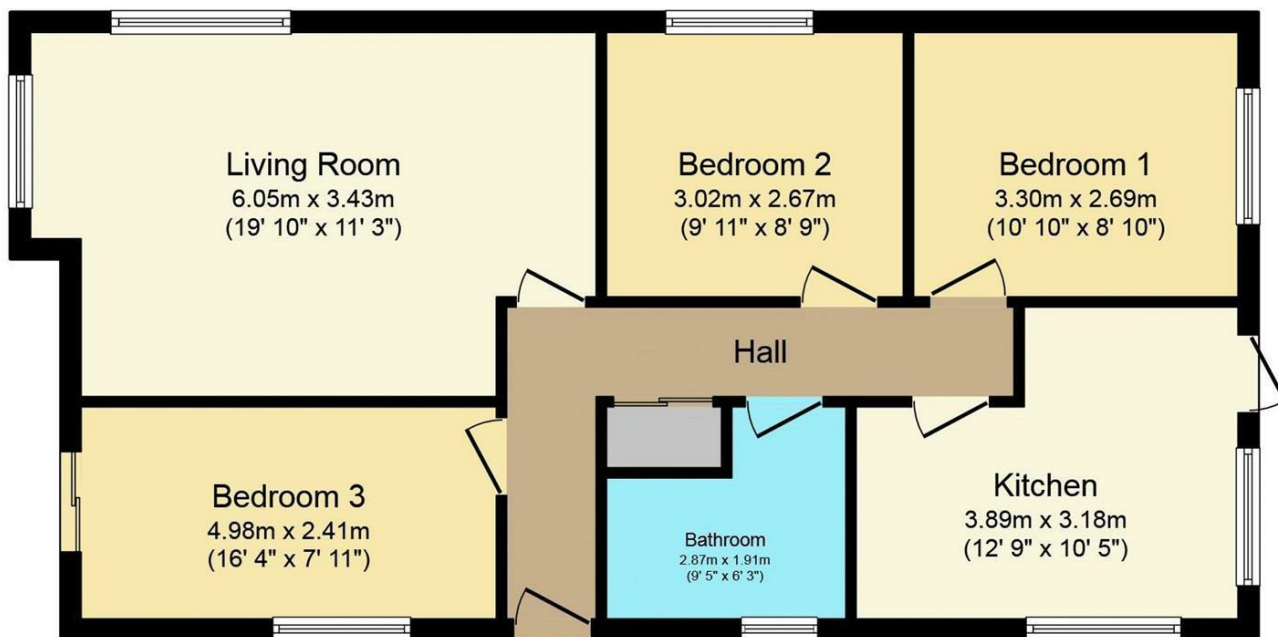
Floor Plan
