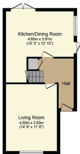
Ground Floor Floor area 41.3 sq.m. (444 sq.ft.) approx
