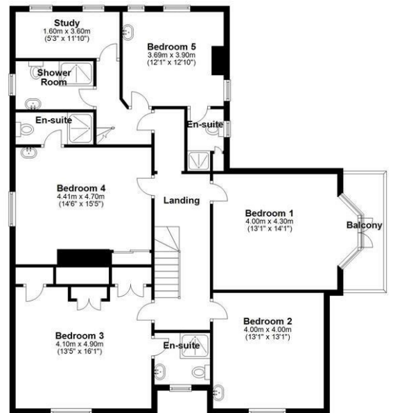
First Floor Approx. 127.3 sq. metres (1370.7 sq. feet)
