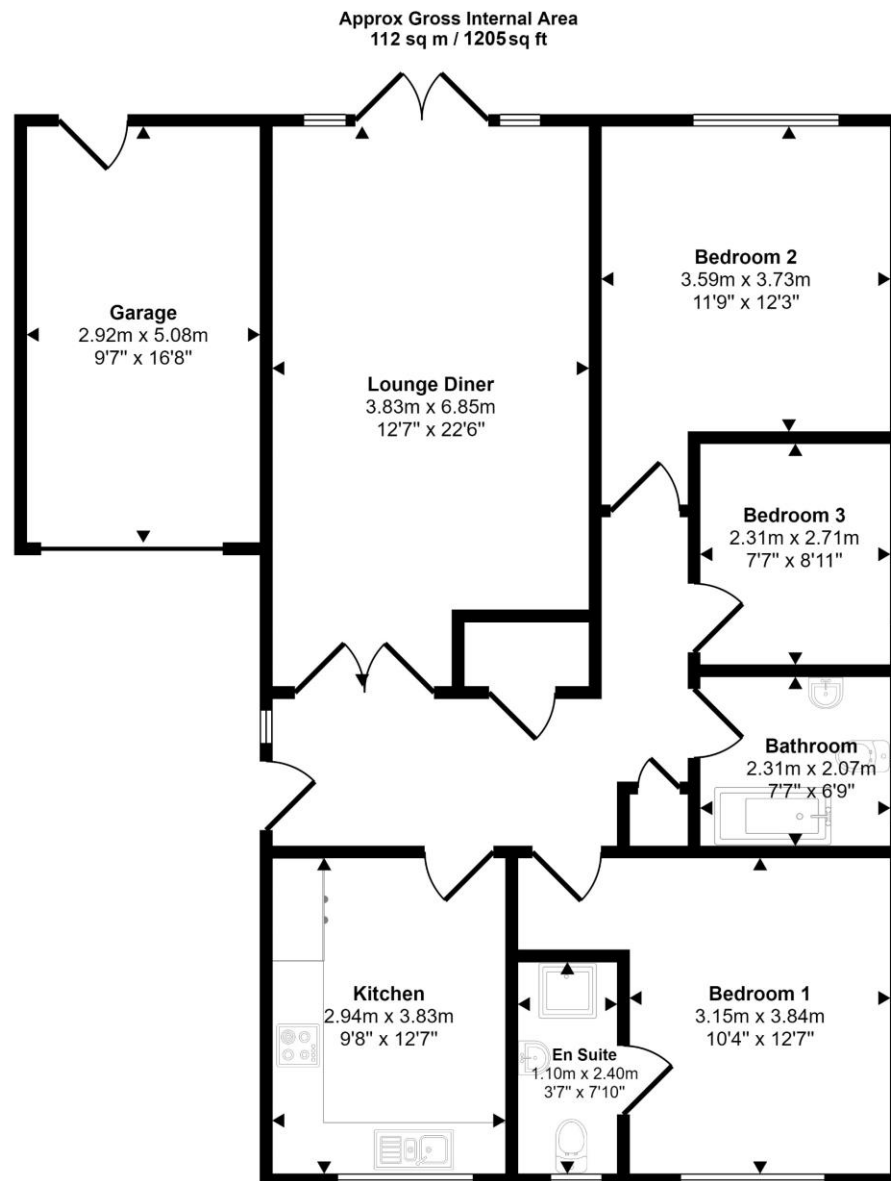
Floorplan
