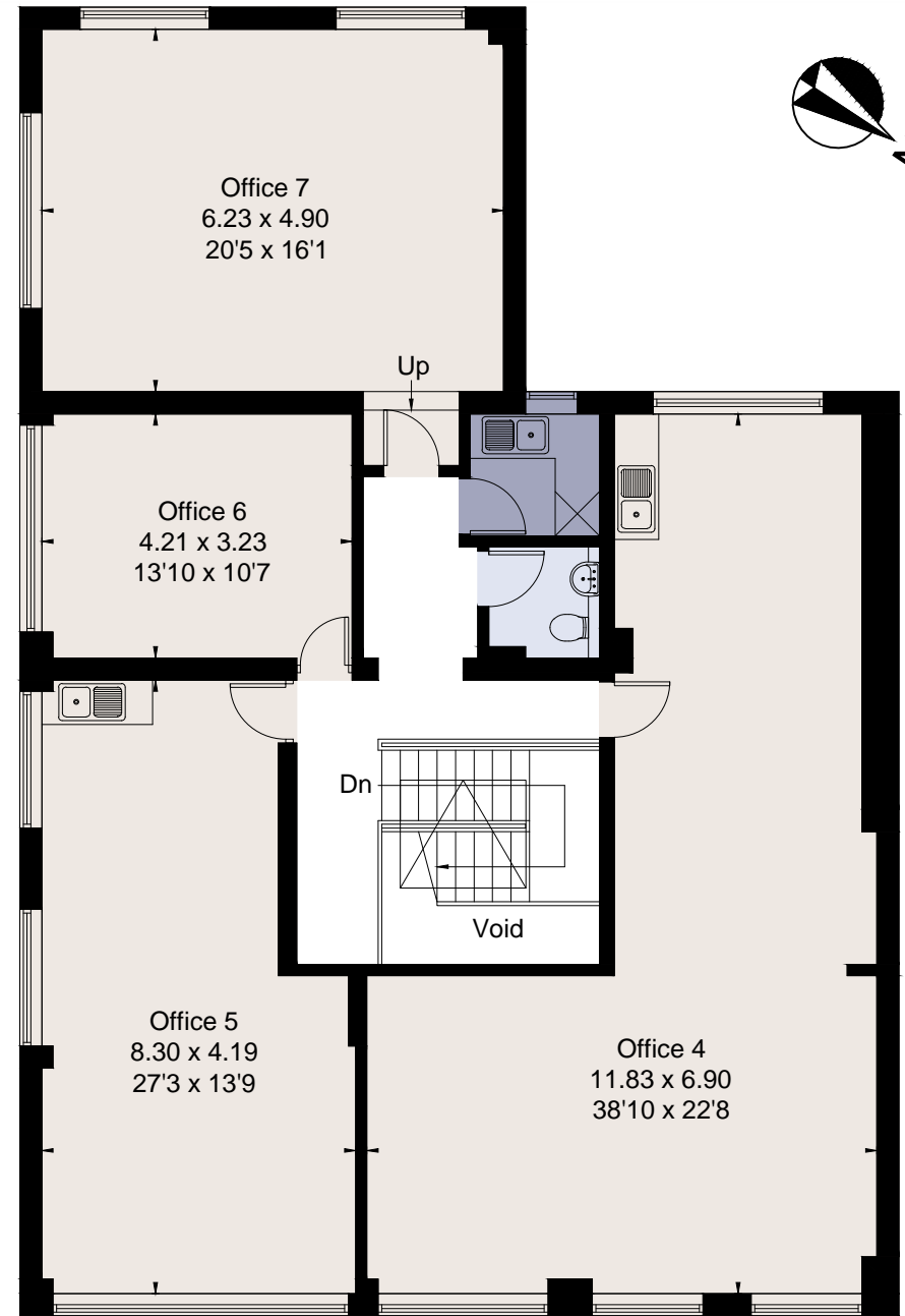
First Floor
