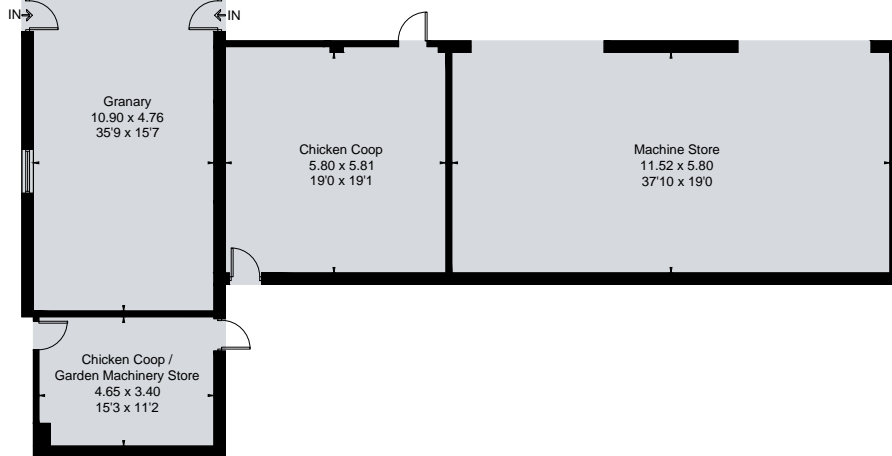
Outbuilding - Ground Floor
