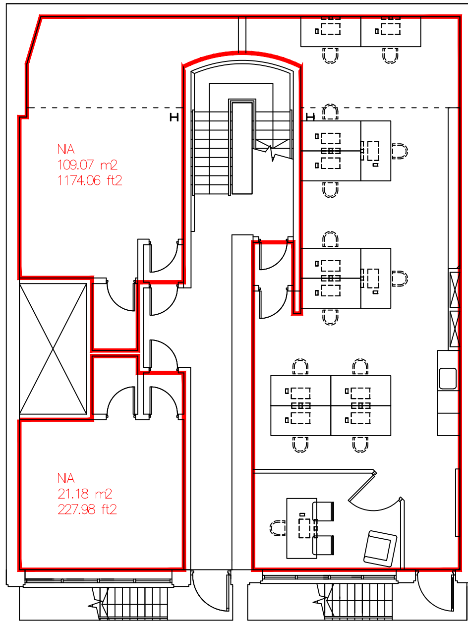
0 1 2 3 4 5 m BASEMENT FLOOR PLAN areas subject to survey (GIA): 1,850 sq ft
