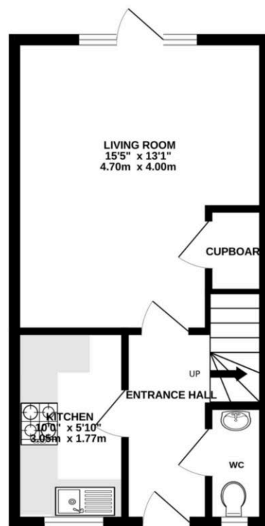
GROUND FLOOR 334 sq.ft. (31.0 sq.m.) approx.
