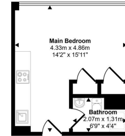
Floorplan
