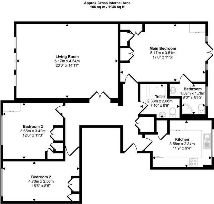
Floorplan
