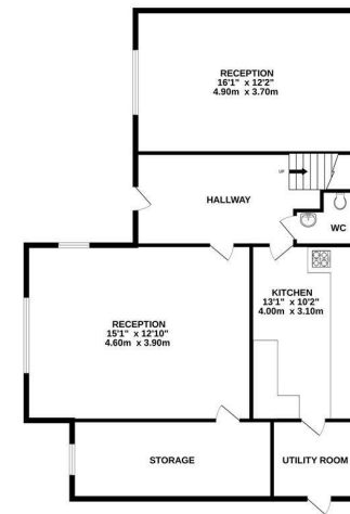
GROUND FLOOR 764 sq.ft. (71.0 sq.m.) approx.
