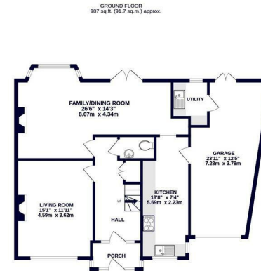
GROUND FLOOR 987 sq. ft. (91.7 sq.m.) approx.
