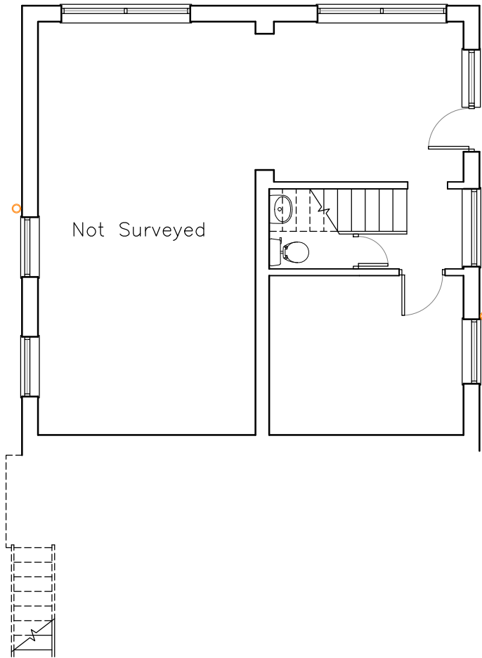
GROUND FLOOR 1:100
