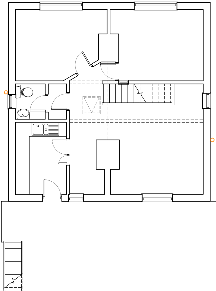
FIRST FLOOR 1:100
