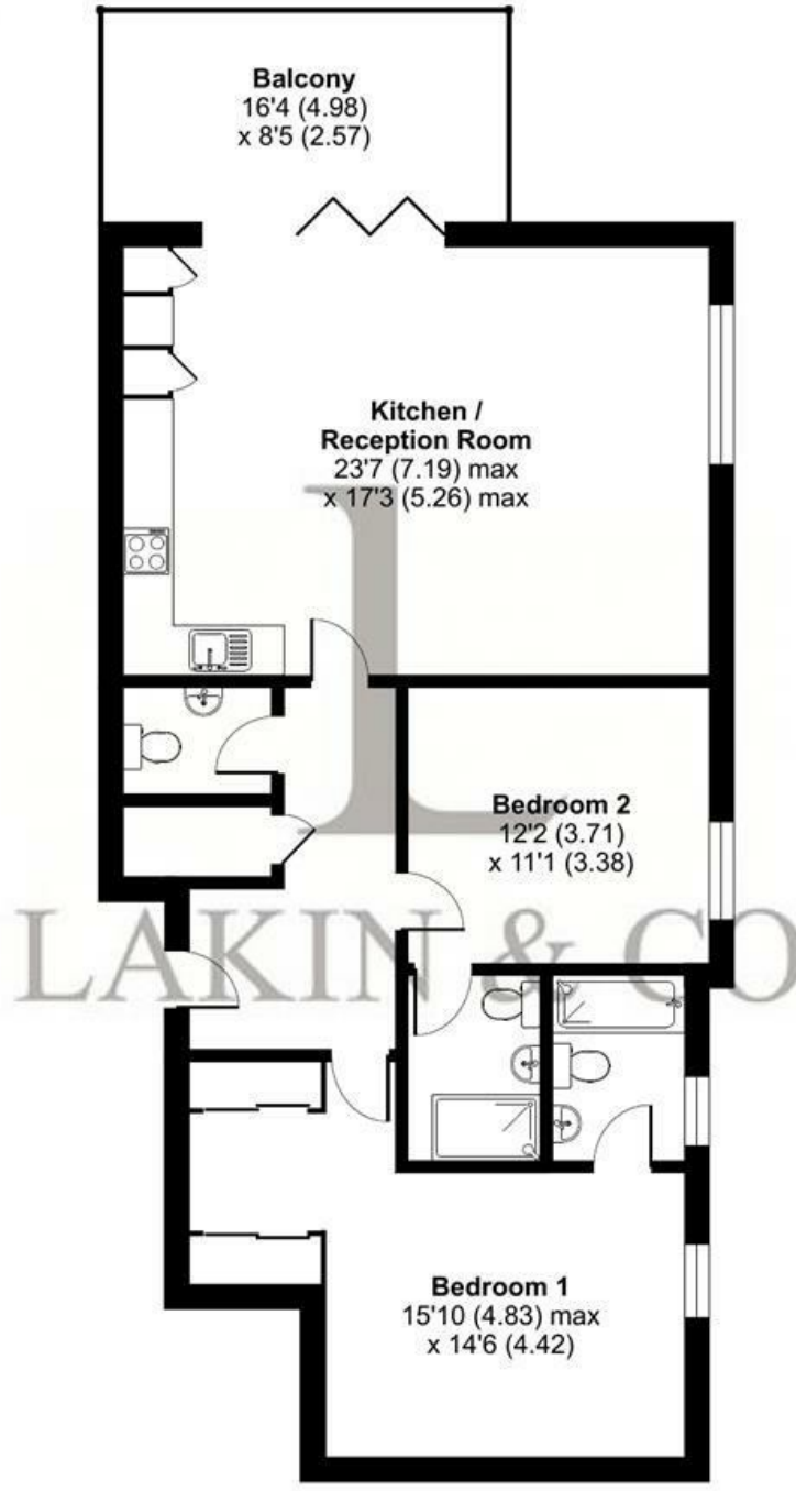
FIRST FLOOR
