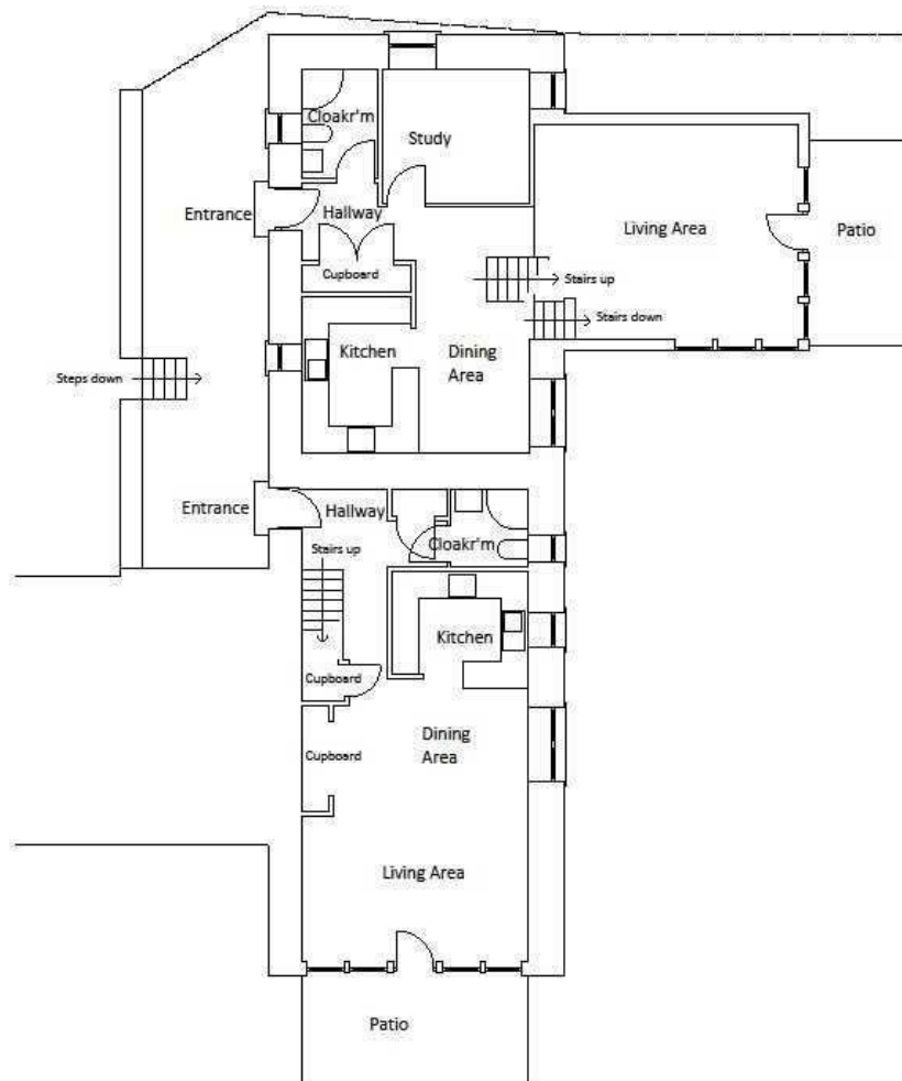
Ground Floor Plan as Proposed Scale 1:100
