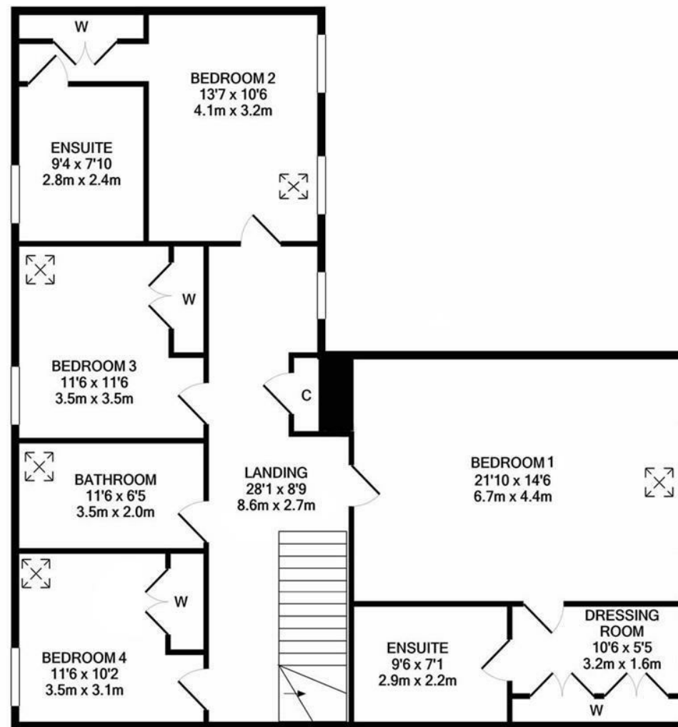
1ST FLOOR
