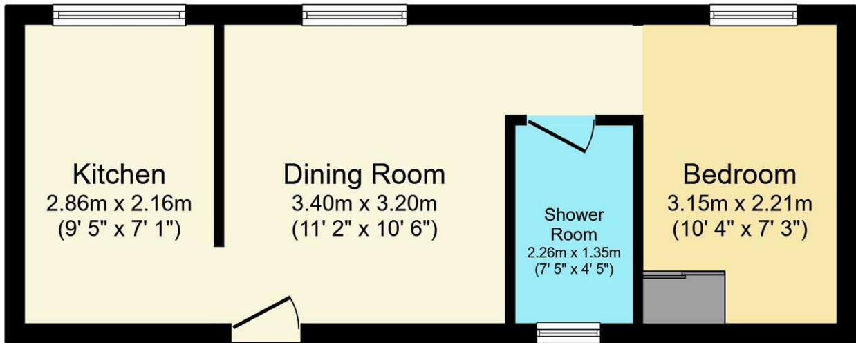
Floor Plan Floor area 31.3 sq.m. (337 sq.ft.)
