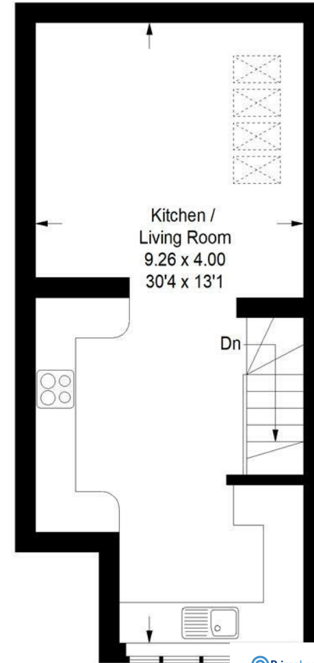
First Floor
