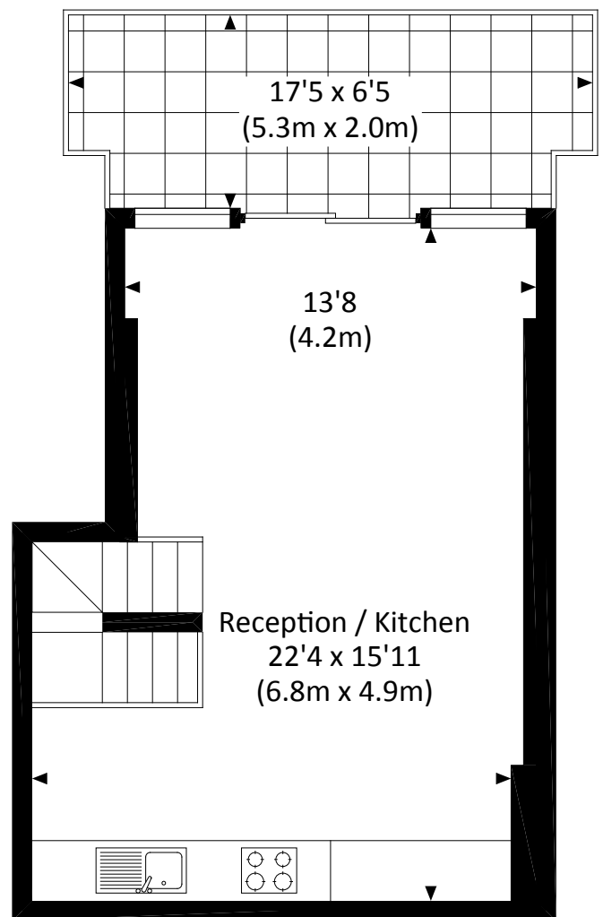
FIRST FLOOR
