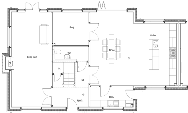
PLOT 1 BROADACRE HOUSE 2357 SQ.FT
