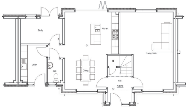
PLOT 2 HAZELDENE HOUSE 1733 SQ.FT
