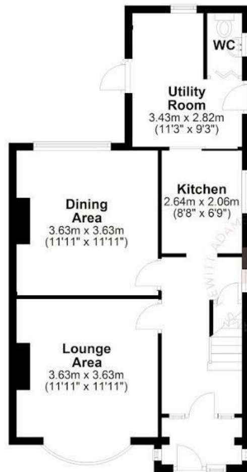
Ground Floor Approx. 54.5 sq. metres (586.4 sq. feet)
