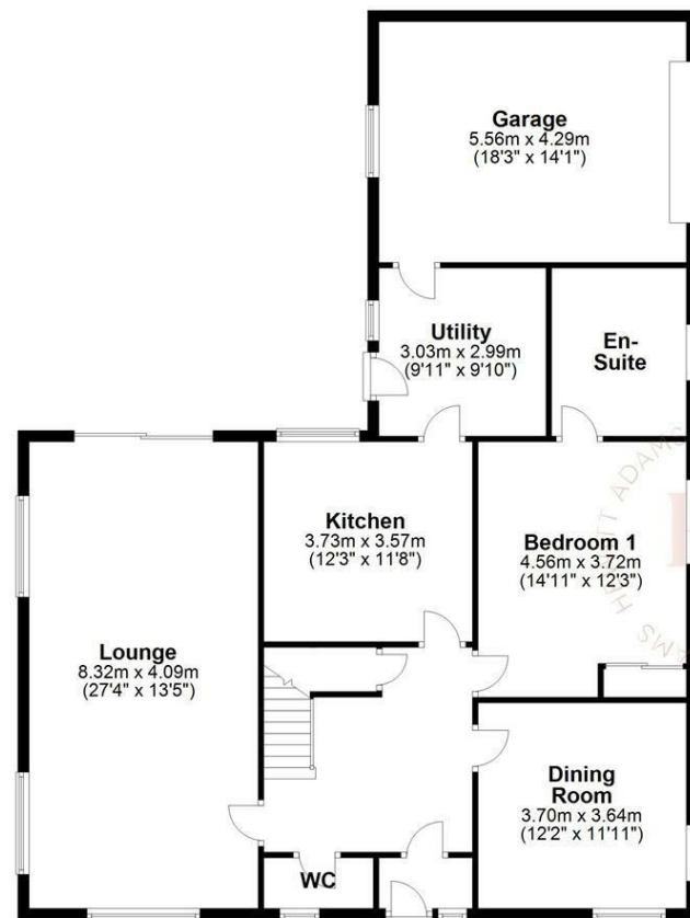
Ground Floor Approx. 139.1 sq. metres (1497.3 sq. feet)
