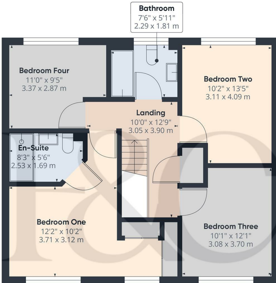
Floor 1 Building 1
