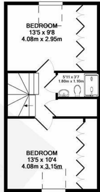
2ND FLOOR APPROX. FLOOR AREA 345 SQ.FT. (32.1 SQ.M.)
