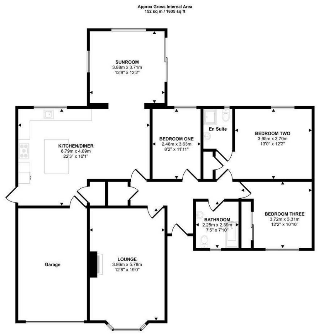
Floorplan
