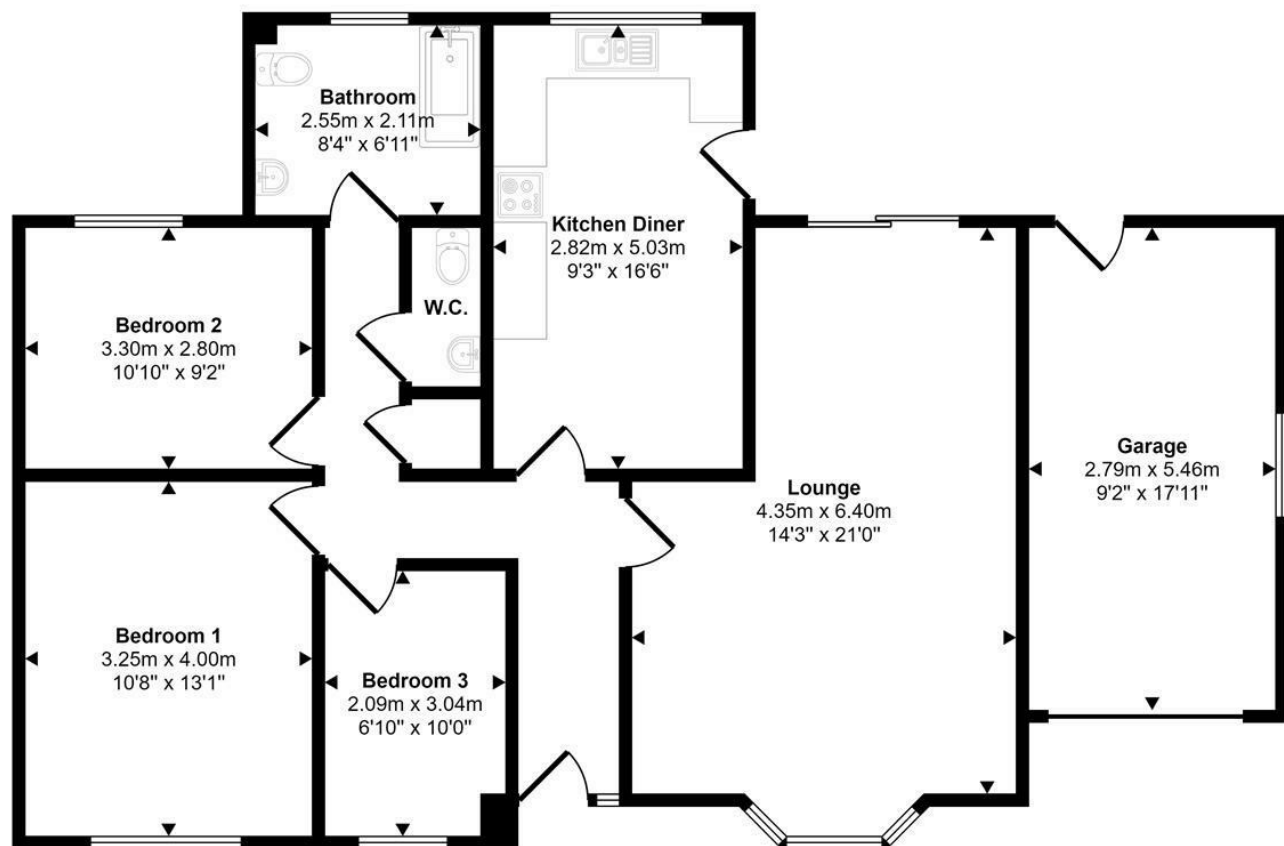
Floorplan
