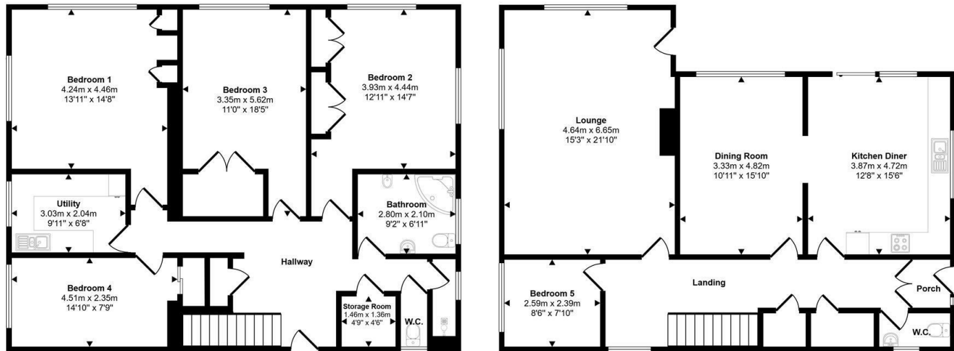
Lower Ground Floor Approx 111 sq m / 1195 sq ft
