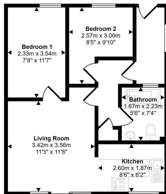
Floorplan
