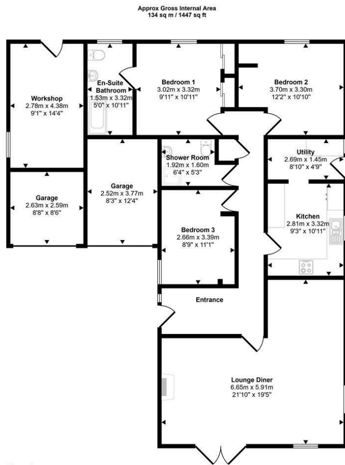
Floorplan
