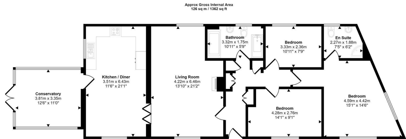
Floorplan
