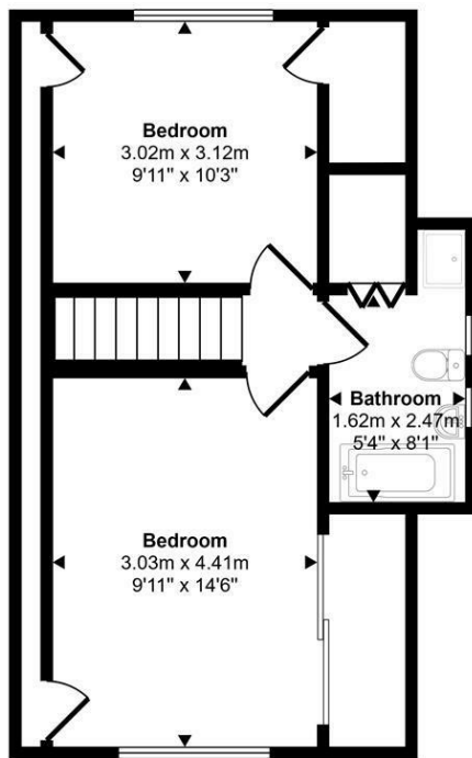
First Floor Approx 41 sq m / 441 sq ft
