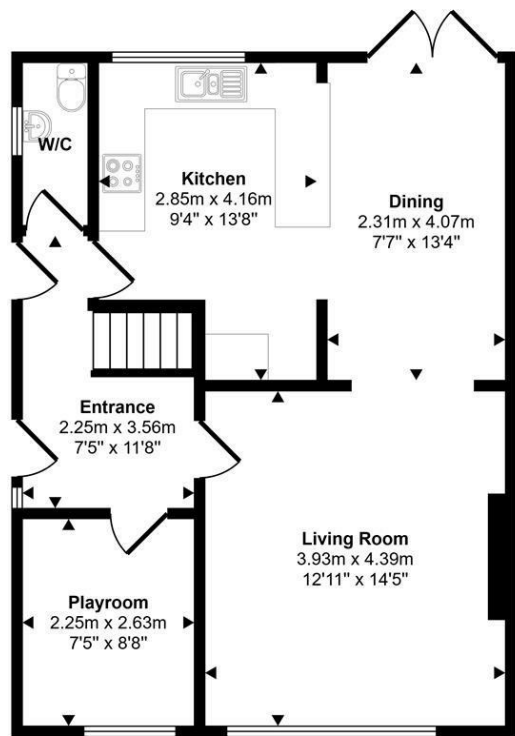
Ground Floor Approx 54 sq m / 585 sq ft
