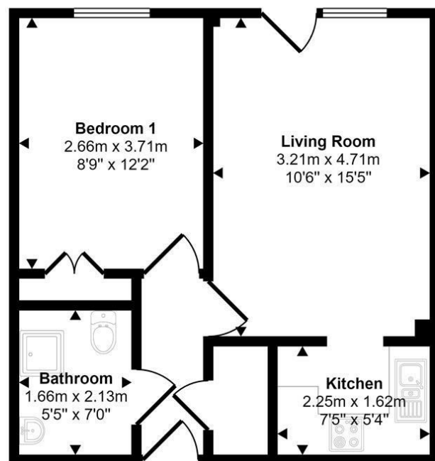
Floorplan
