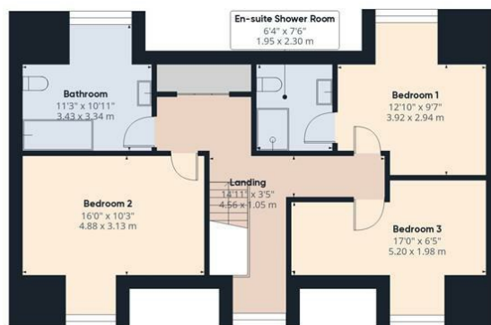
Floor 2
