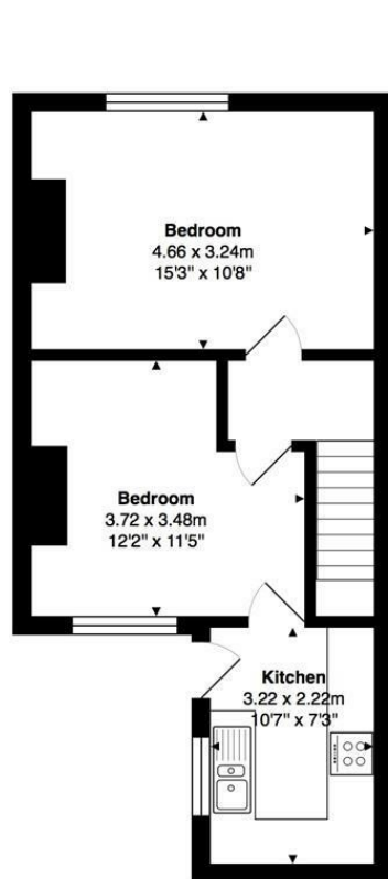
Lower Ground Floor Area: 39.6 m 2 ... 426 ft 2
