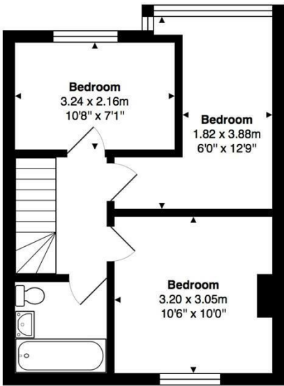
First Floor Area: 36.1 m 2 ... 389 ft 2
