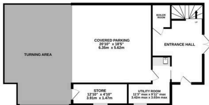
GROUND FLOOR 731 sq.ft. (67.9 sq.m.) approx.
