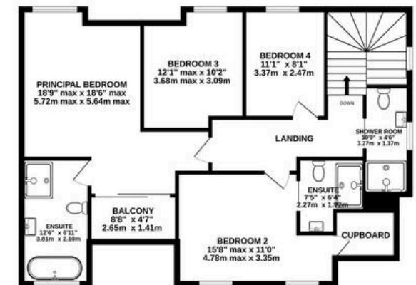
2ND FLOOR 1028 sq.ft. (95.5 sq.m.) approx.
