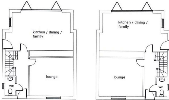
PROPOSED GROUND FLOOR PLAN 1:100
