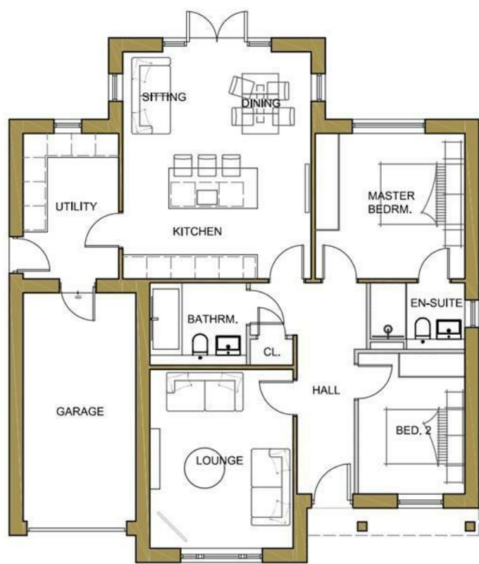
FLOOR PLAN 95.98m 2 G.L.A. (1033 sq. ft) 24m garage @ 15.89m 2 G.L.A. (171 sq. ft.)
