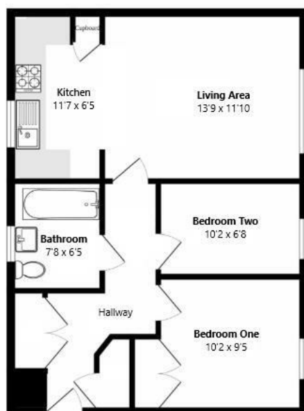
Ground Floor Apartment 567 ft 2 (52m 2 )
