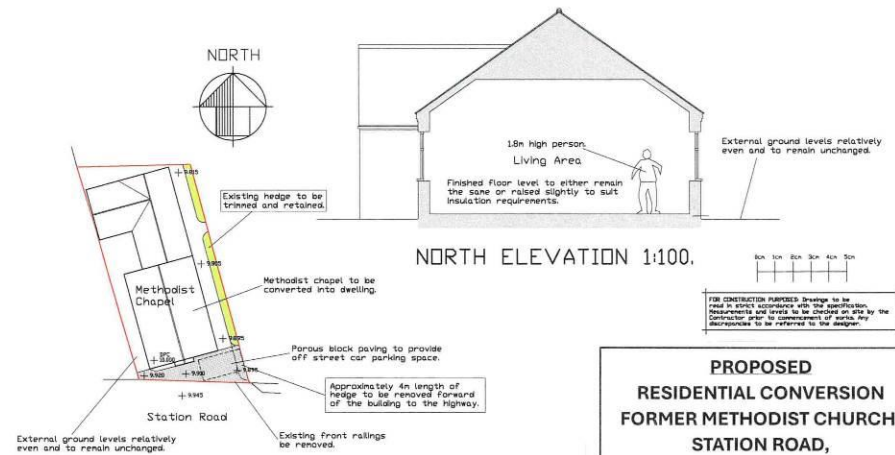
NORTH ELEVATION 1:100.
