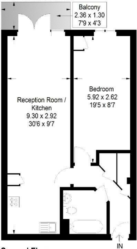
Second Floor
