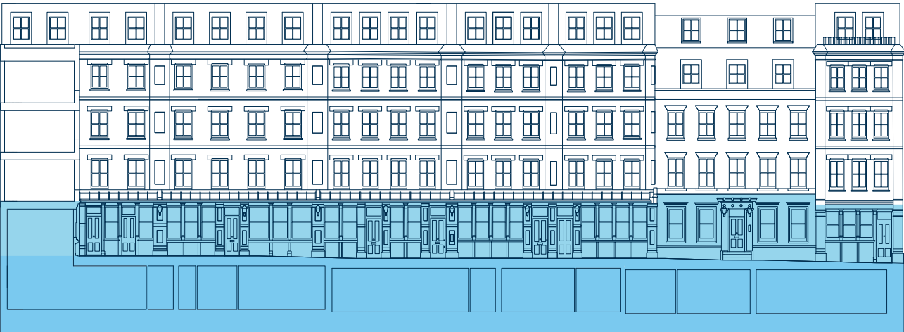
West Elevation
