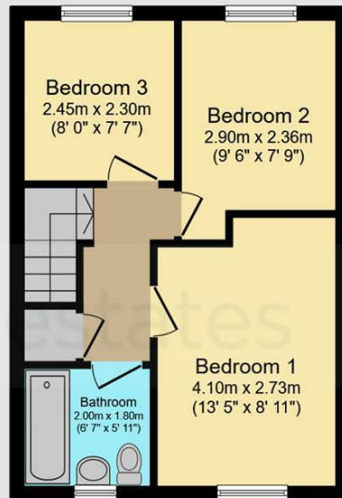
First Floor Floor area 33.8 m 2 (364 sq.ft.)
