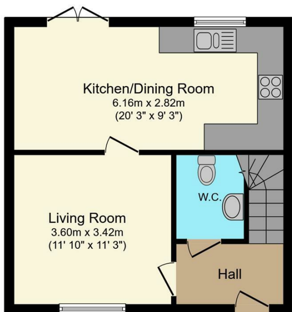
Ground Floor Floor area 39.0 m 2 (420 sq.ft.)
