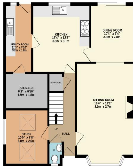
GROUND FLOOR 757 sq.ft. (70.3 sq.m.) approx.
