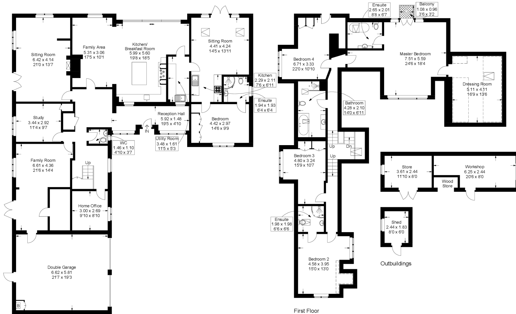
First Floor
